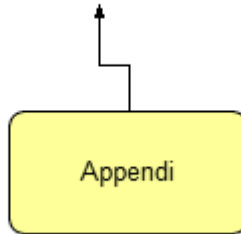
Appendi
